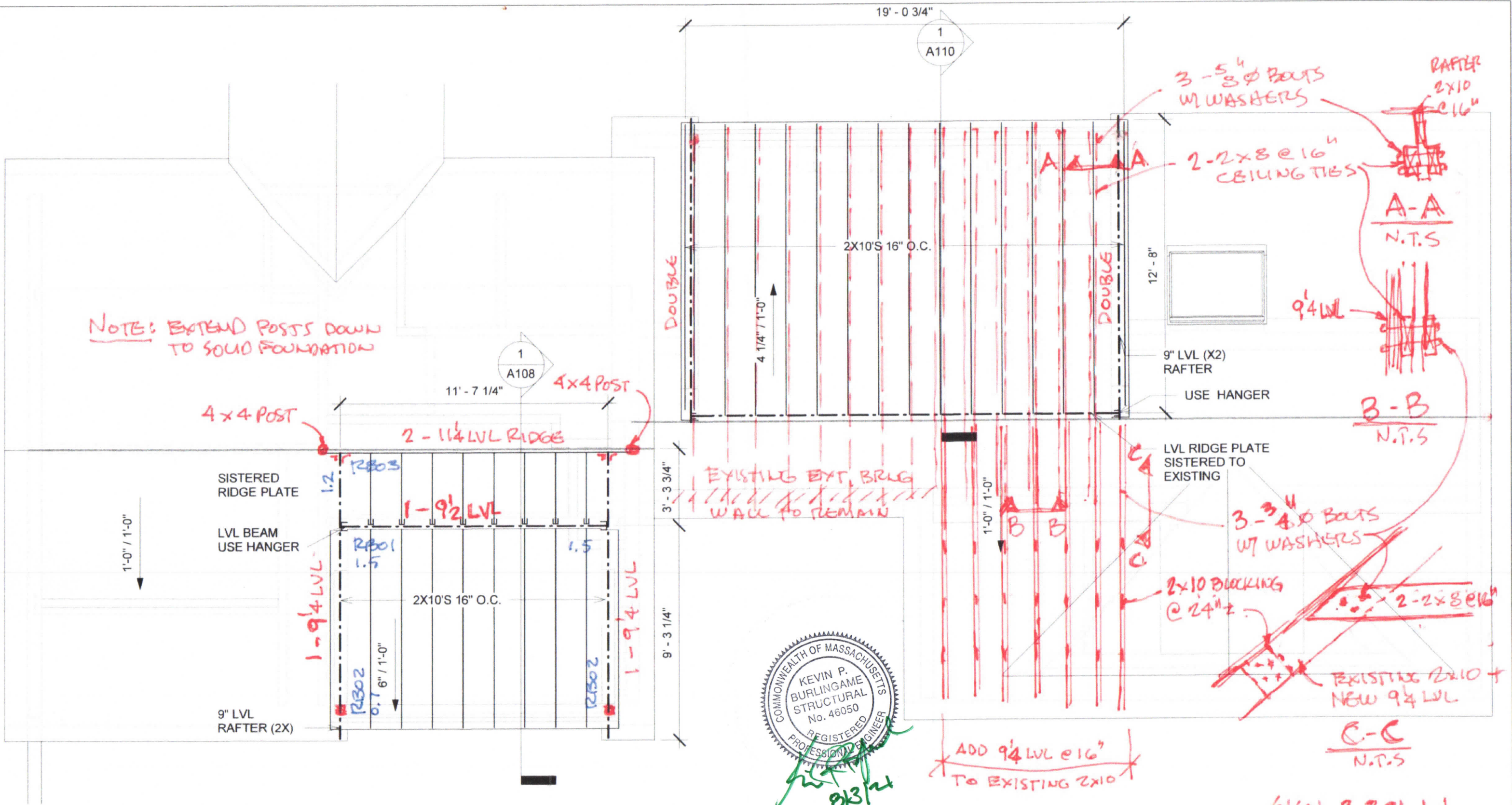
1 ROOF PEAK - FRAMING 1/4" = 1'-0"
