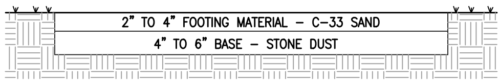
HORSE PADDOCK/RIDING AREA CROSS SECTION NOT TO SCALE
