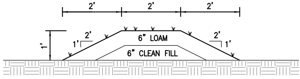
BERM DETAIL NOT TO SCALE
