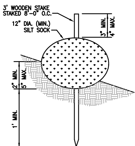
STAKED SILT SOCK DETAIL NOT TO SCALE
