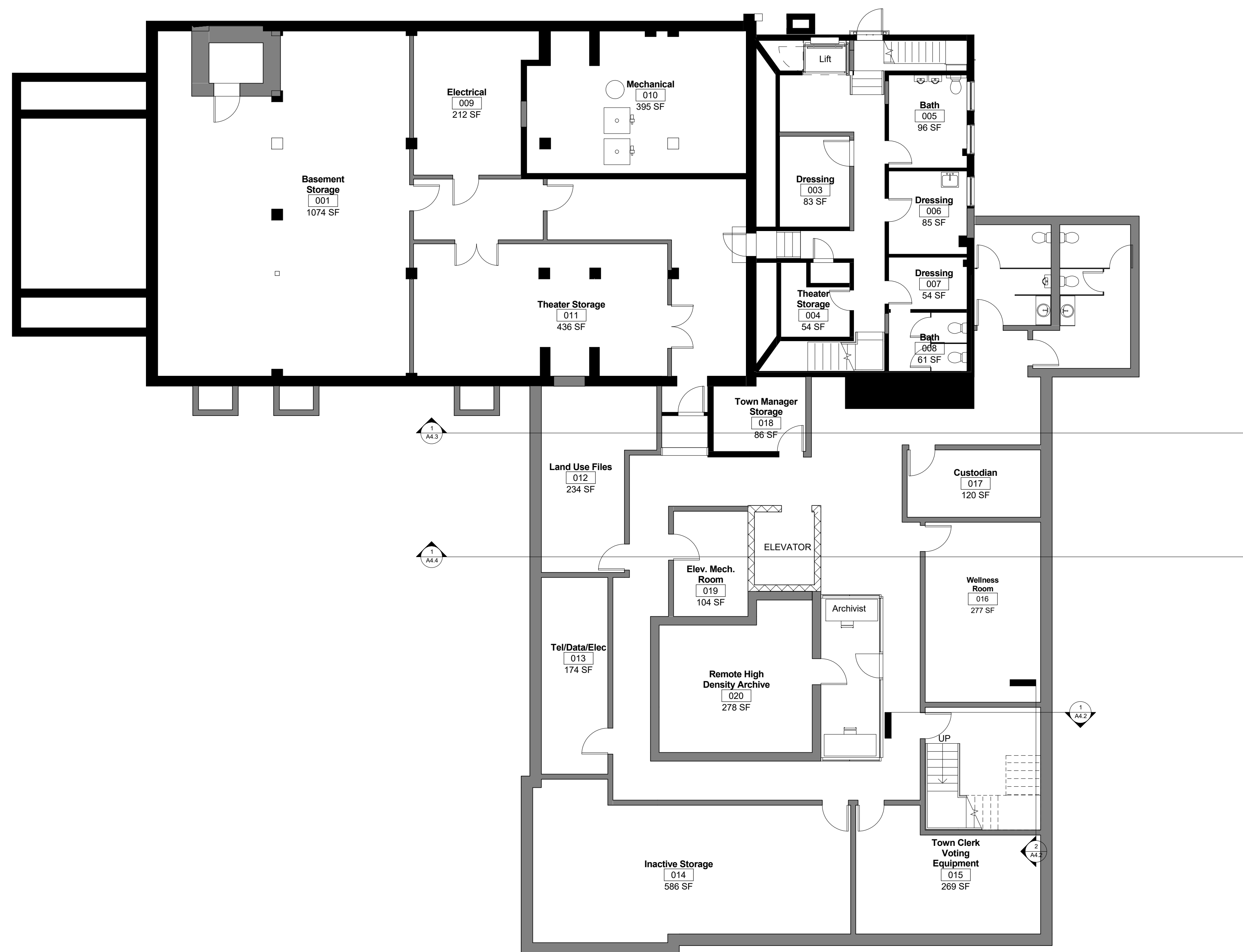
1 Basement - Scheme 3 1/8" = 1'-0"
