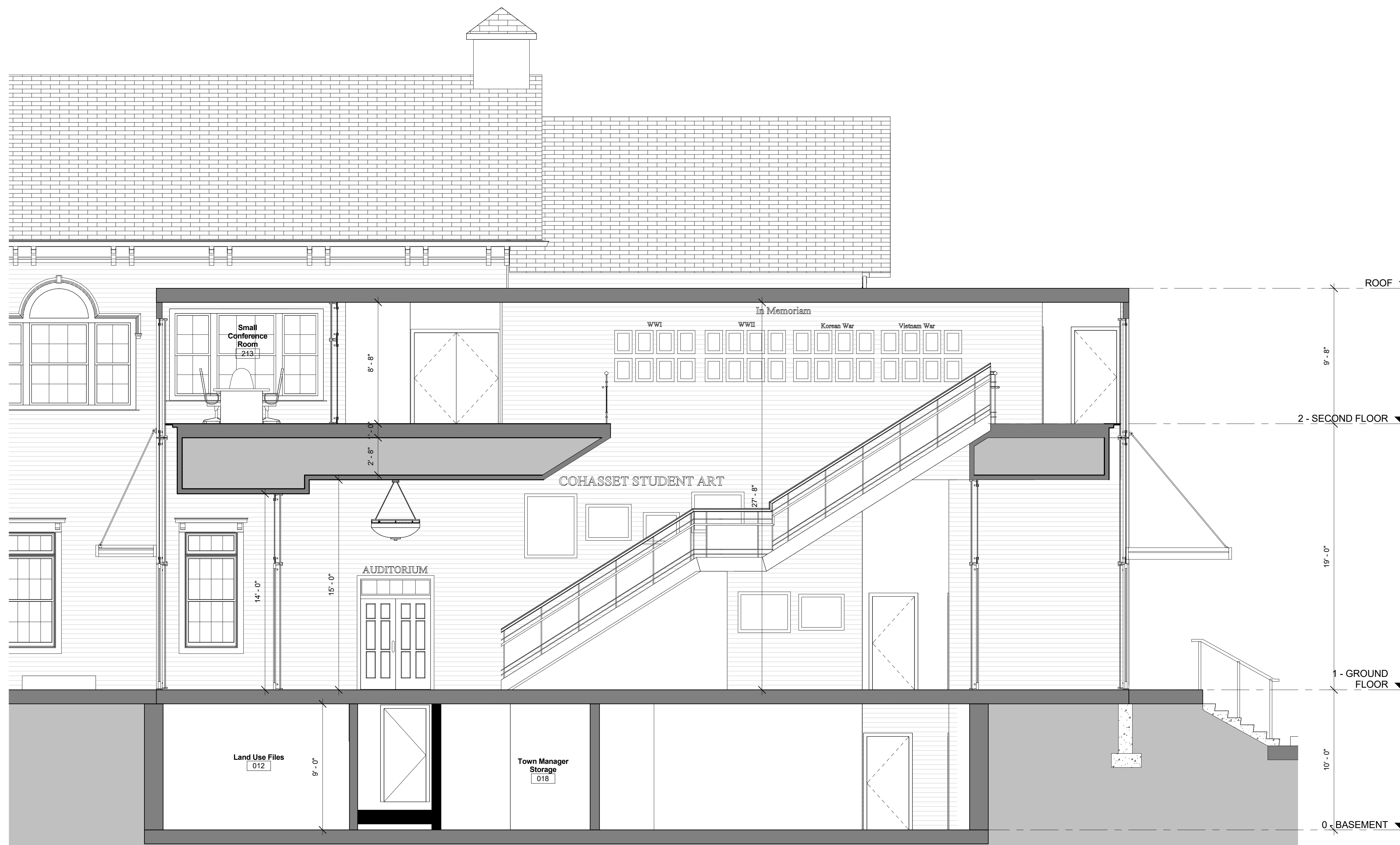
1 East West Section 1/4" = 1'-0"
