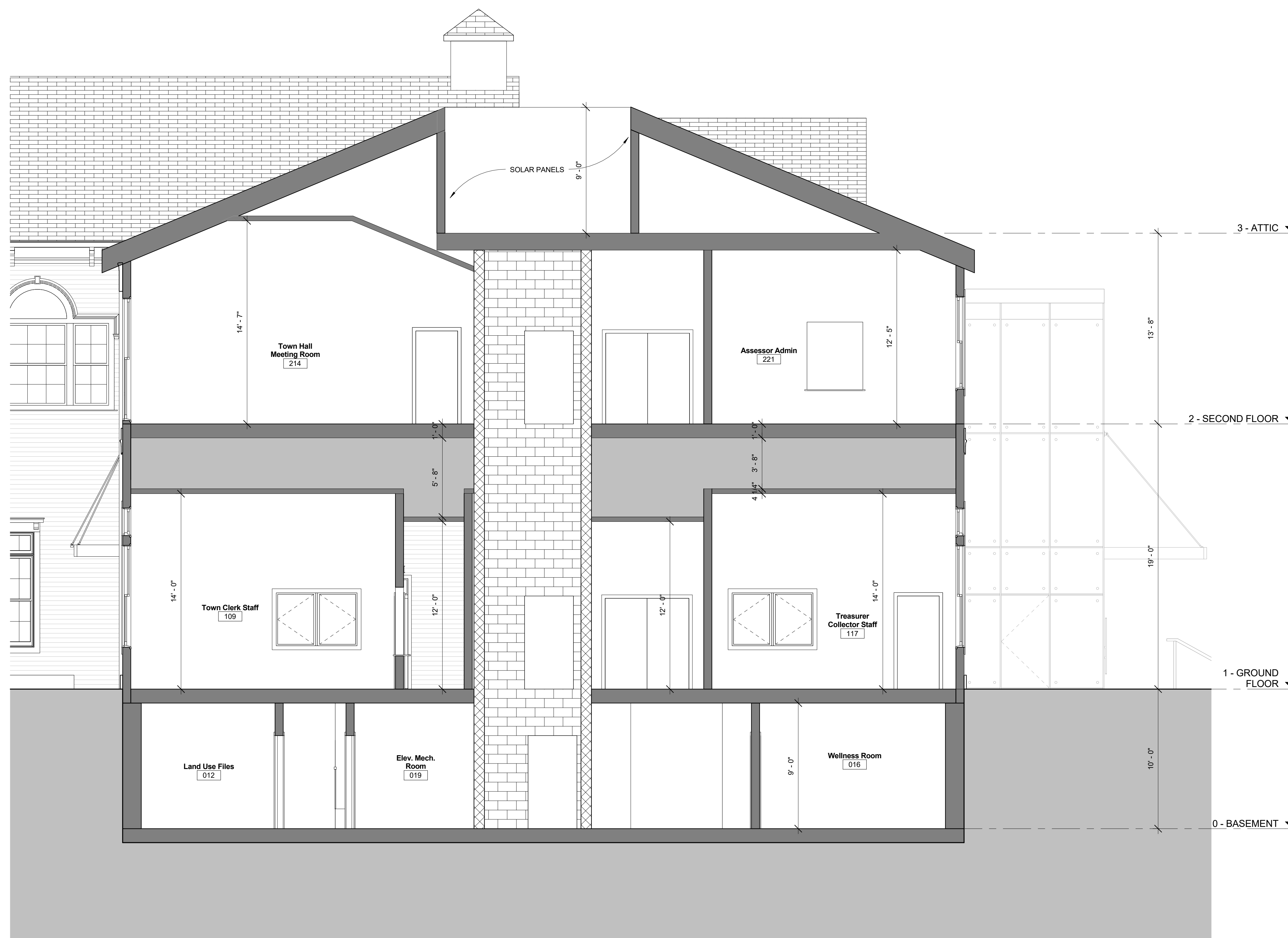
1 Cross Section 1/4" = 1'-0"
