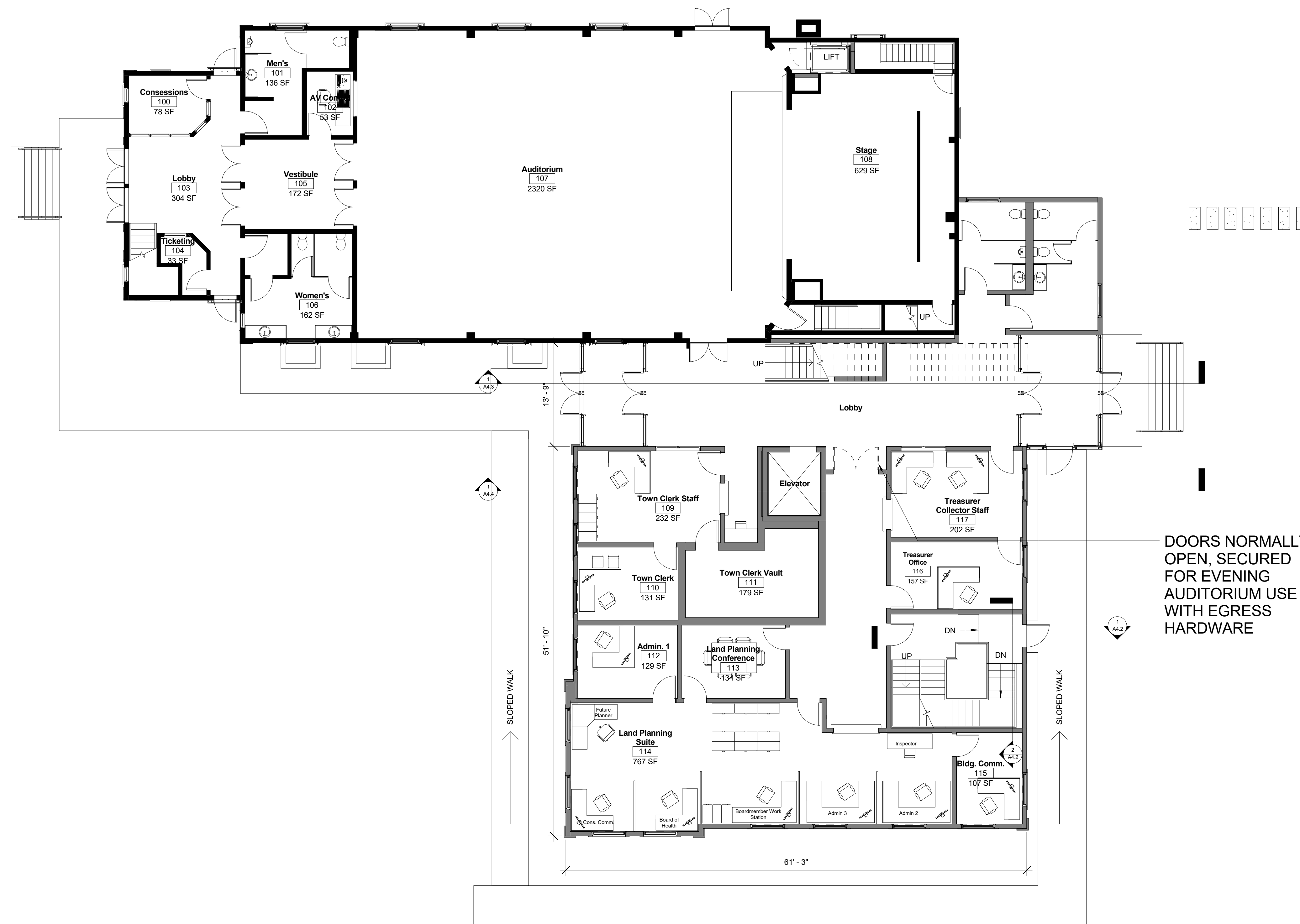
1 First Floor-Scheme 3 1/8" = 1'-0"
